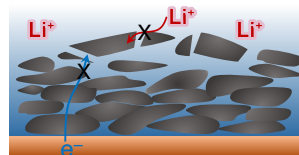
Mechanical deformation
