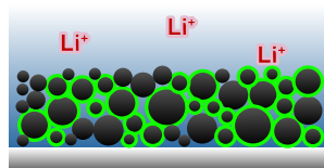
Percolation-limited connectivity
